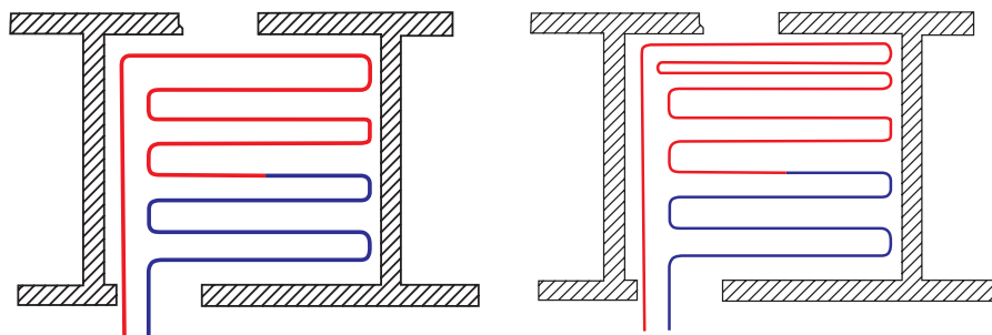
Meander bedding without/with peripheral zones
