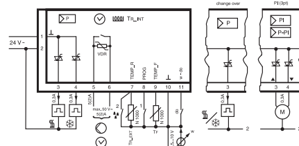
Connection plan, 24 V version, 1 7794 24
