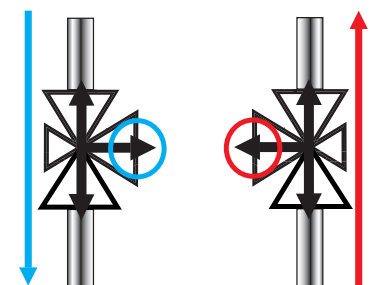
1/2 Outlet is shut off Multi-functional opening Shut-off for maintenance/ changing
