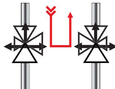
"Up" is accessible "Down" shut-off "Flush top"
