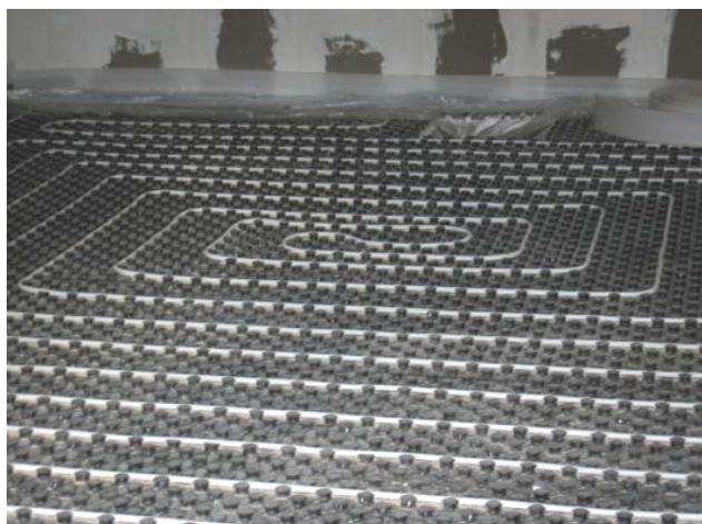
Spiral control with pimples plate
