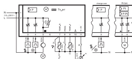
Connection plan, 230 V version, 1 7794 23
