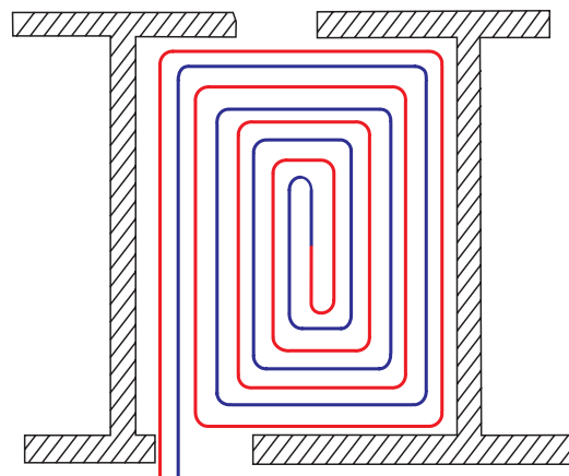
Spiral bedding
