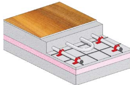
Recommended clip interval, 300-500 mm Bending radius 5 x D
